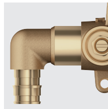
1/2" PEX cold expansion (ASTM F1960) elbow inlets
