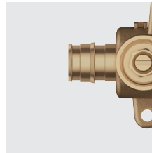
1/2" PEX cold expansion (ASTM F1960) inlets
