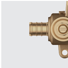
1/2" PEX crimp (ASTM F1807) inlets
